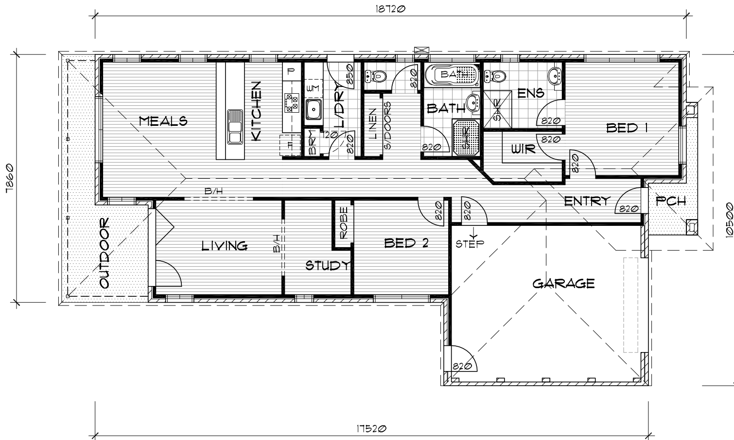
FLOOR PLAN
